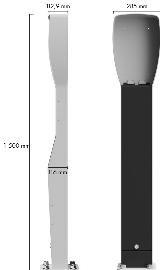
ZapCharger Single Column Premium
