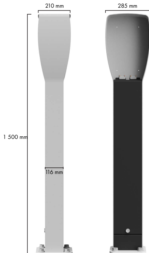
ZapCharger Twin Column Premium
